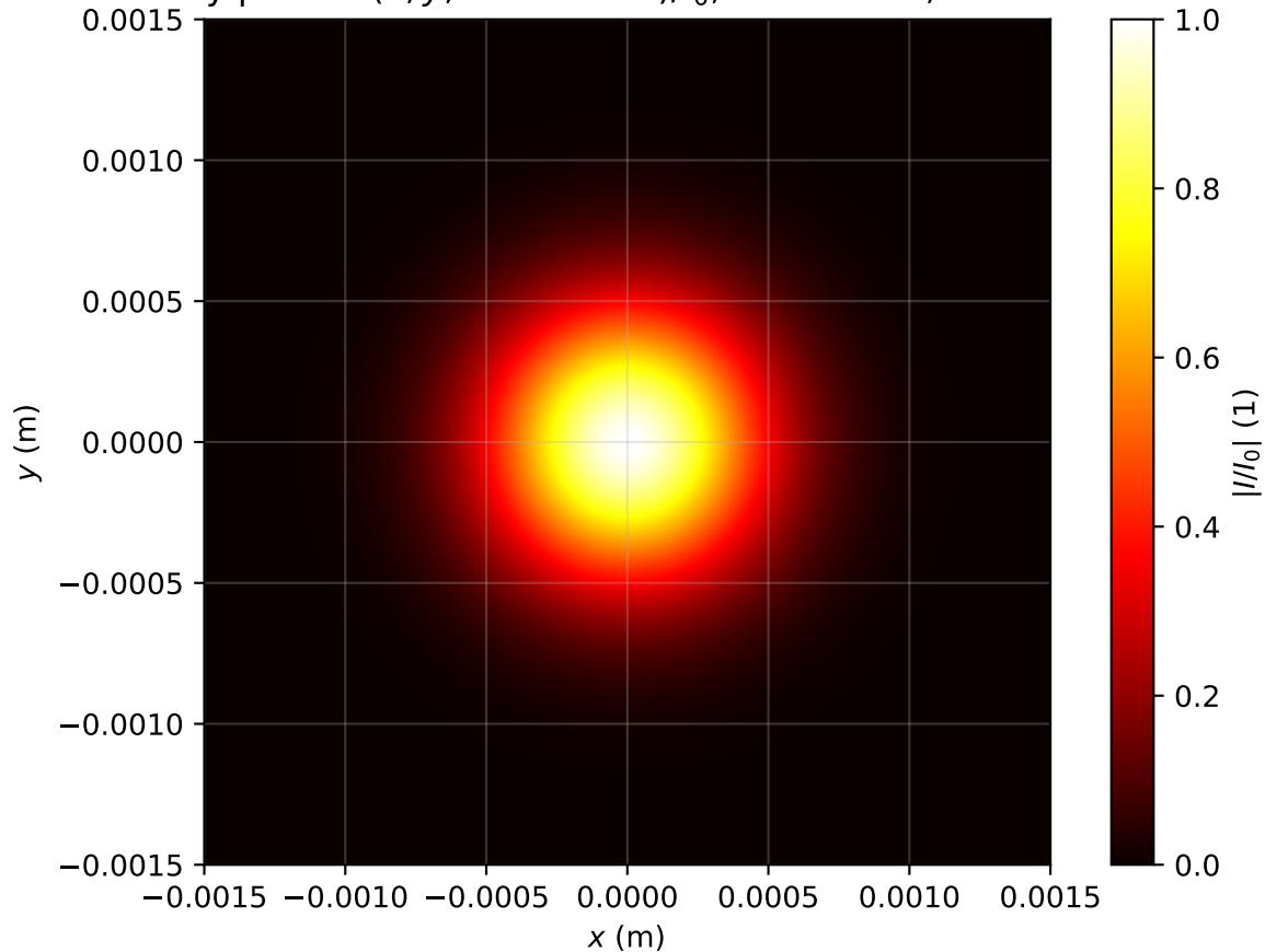
Intensity profile I(x, y, z = 0.000\text{m})/I_0 , Pin=1.0Pcr, artificial time
